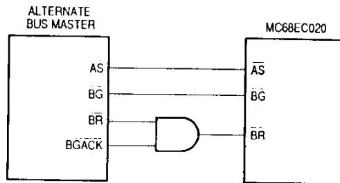
Figure 5-50. Interface for Three-Wire to Two-Wire Bus Arbitration
