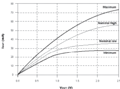
FIGURE C – PULL-DOWN CHARACTERISTICS
