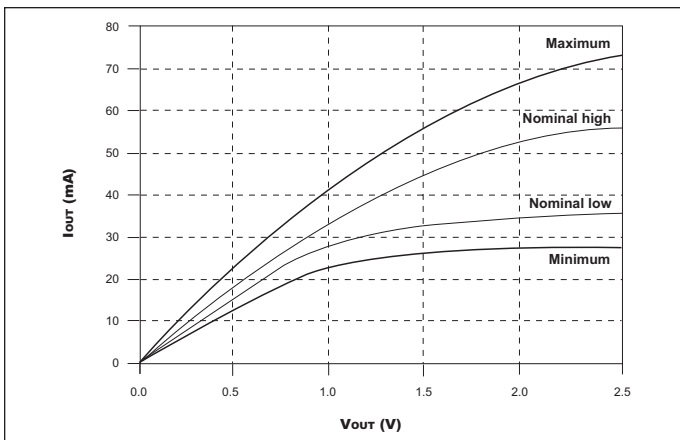
FIGURE C – PULL-DOWN CHARACTERISTICS
