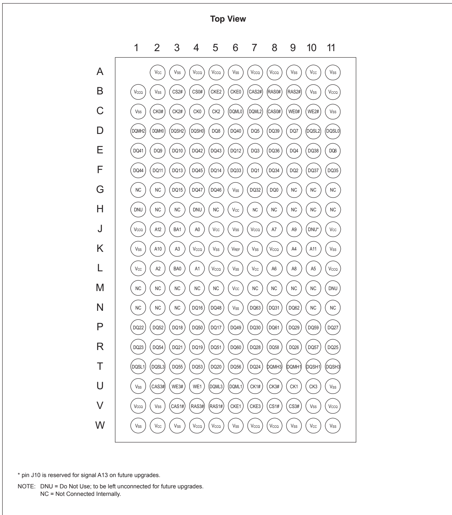
FIGURE 1 – PIN CONFIGURATION
