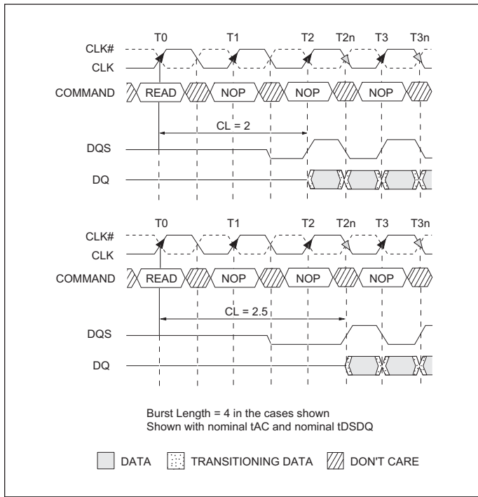
FIGURE 4 – CAS LATENCY
