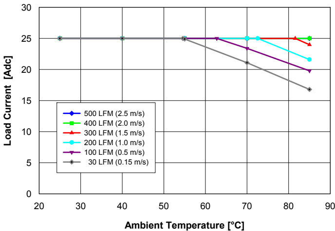
Fig. 1: Available load current vs. ambient air temperature and air flow rates for Q24T25025 converter mounted vertically with air flowing from pin 3 to pin 1, MOSFET temperature \leq 120^{\circ}\text{C} , V_{in} = 27\text{ V} .
