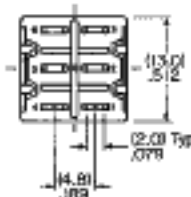
M2011 & M2021 models do not have terminals 1 & 4.
