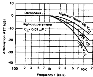
ATT-f (Graph 7)
