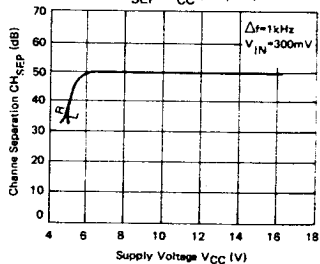
CH<sub>SEP</sub>-V<sub>CC</sub> (Graph 4)
