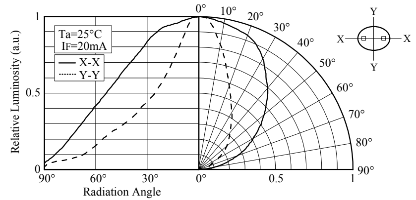
■ Directivity (NSPR346BS)
