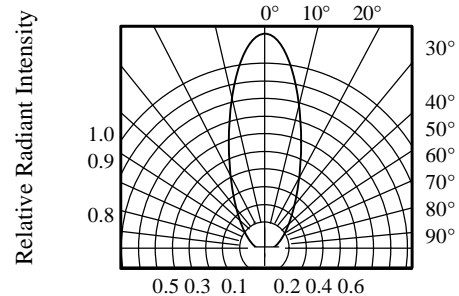
FIG.5 RADIATION DIAGRAM
