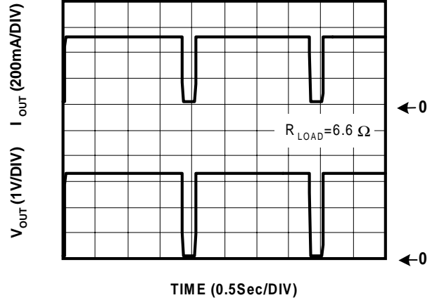
Overtemperature Shutdown
