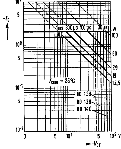
Permissible operating range I_C = f(V_{CE}); (T_{case} = 60^\circ\text{C}); v = 0 BD 136, BD 138, BD 140
