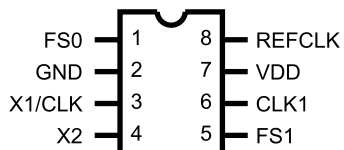
AV9107C-05/-10 8-Pin DIP, SOIC
