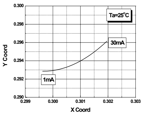
CIE Diagram vs Forward Current
