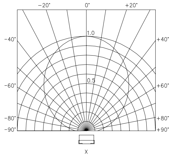
Radiation Diagram
