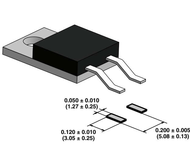
FIGURE 6 - VPR220S LAND PATTERN DIMENSIONS in inches (millimeters)
