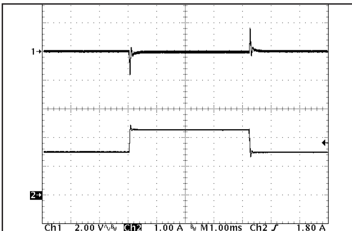
Figure 5: Output voltage response to step-change in load current (66%-100%-66% of I out (max); dI/dt = 0.05A/μs). Load cap: 1μF ceramic cap. Ch 1: V out (2V/div), Ch 2: I out (1A/div).
