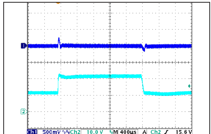
Figure 6: Output voltage response to step-change in input voltage (250 V/ms). Load cap: 100µF electrolytic output capacitance. Ch 1: Vout (500mV/div), Ch 2: Vin (10V/div).
