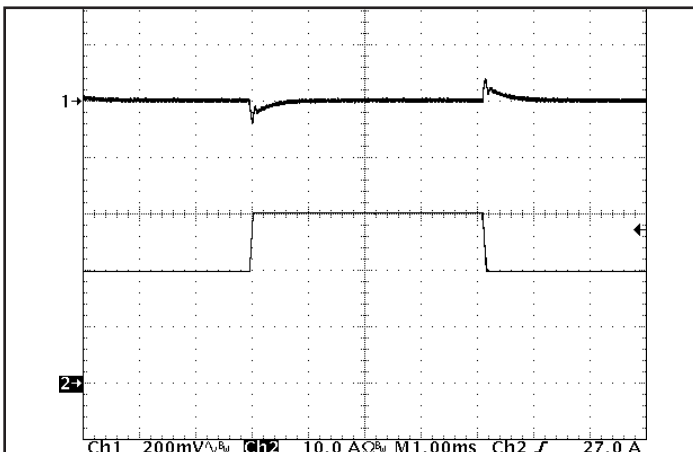
Figure 5: Output voltage response to step-change in load current (66%-100%-66% of Iout(max); dI/dt = 0.2A/us). Load cap: 1µF ceramic cap and 15µF tantalum cap. Ch 1: Vout (200mV/div), Ch 2: Iout (10A/div).
