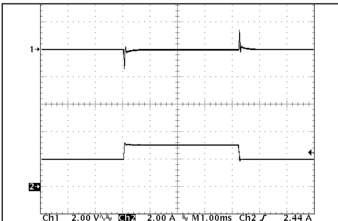
Figure 5: Output voltage response to step-change in load current (66%-100%-66% of I out (max); dI/dt = 0.08A/μs). Load cap: 1μF ceramic cap. Ch 1: V out (2V/div), Ch 2: I out (2A/div).
