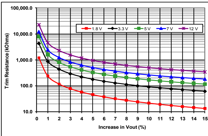
Common Figure 3: Trim-Up Graph for 5.0 to 15V outputs.
