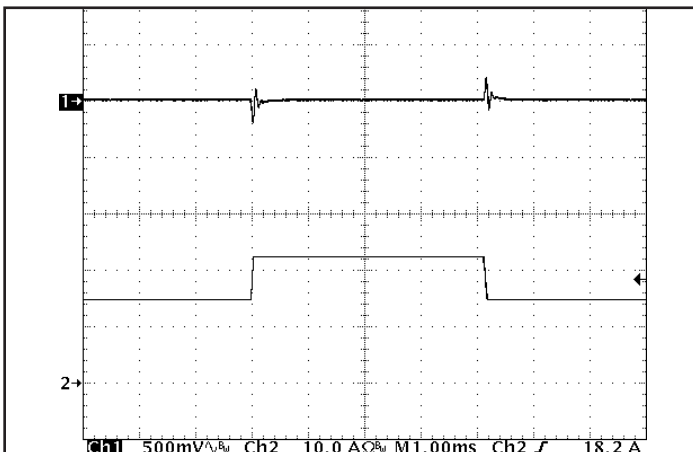
Figure 5: Output voltage response to step-change in load current (66%-100%-66% of I out (max); dI/dt = 0.2A/μs). Load cap: 15μF tantalum cap and 1μF ceramic cap. Ch 1: V out (500mV/div), Ch 2: I out (10A/div).
