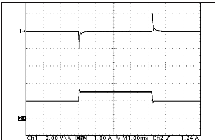
Figure 5: Output voltage response to step-change in load current (66%-100%-66% of I out (max); dI/dt = 0.02A/μs). Load cap: 1μF ceramic cap. Ch 1: V out (2V/div), Ch 2: I out (1A/div).
