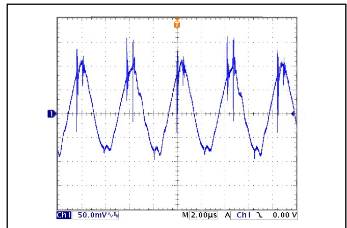
Figure 12: Output voltage ripple at nominal input voltage and rated load current (50 mV/div; 2 \mu\text{s}/\text{div} ). Load capacitance: 1 \mu\text{F} ceramic capacitor and 100 \mu\text{F} electrolytic capacitor. Bandwidth: 20 MHz. See Figure 9.
