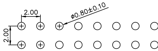
Recommended P.C.B Layout(Top Side) P.C.B Thickness=1.20mm(Tolerance±0.05)
