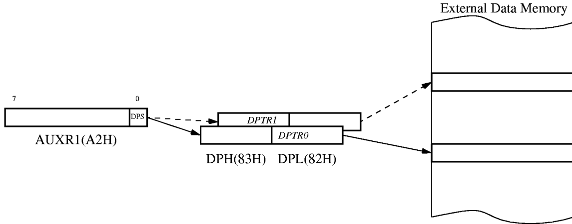
Figure 3. Use of Dual Pointer
