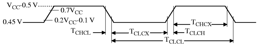
Figure 17. External Clock Drive Waveforms
