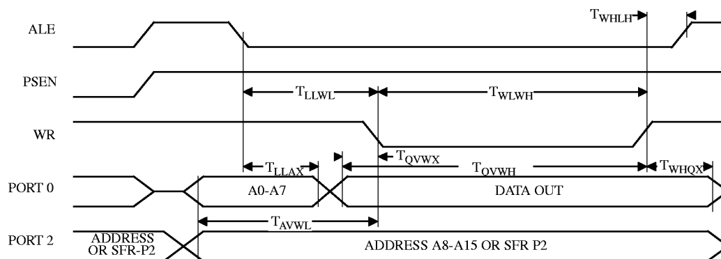
Figure 14. External Data Memory Write Cycle
