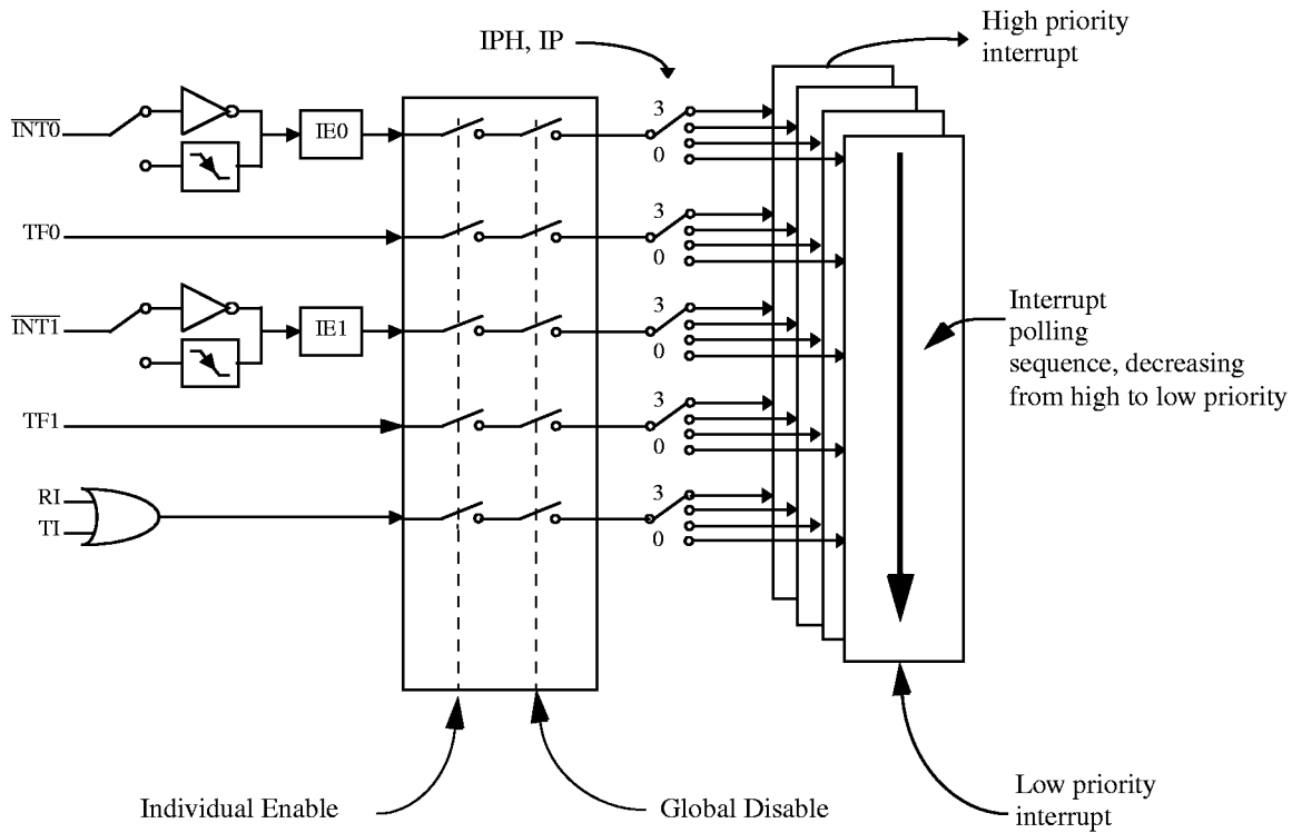
Figure 7. Interrupt Control System
