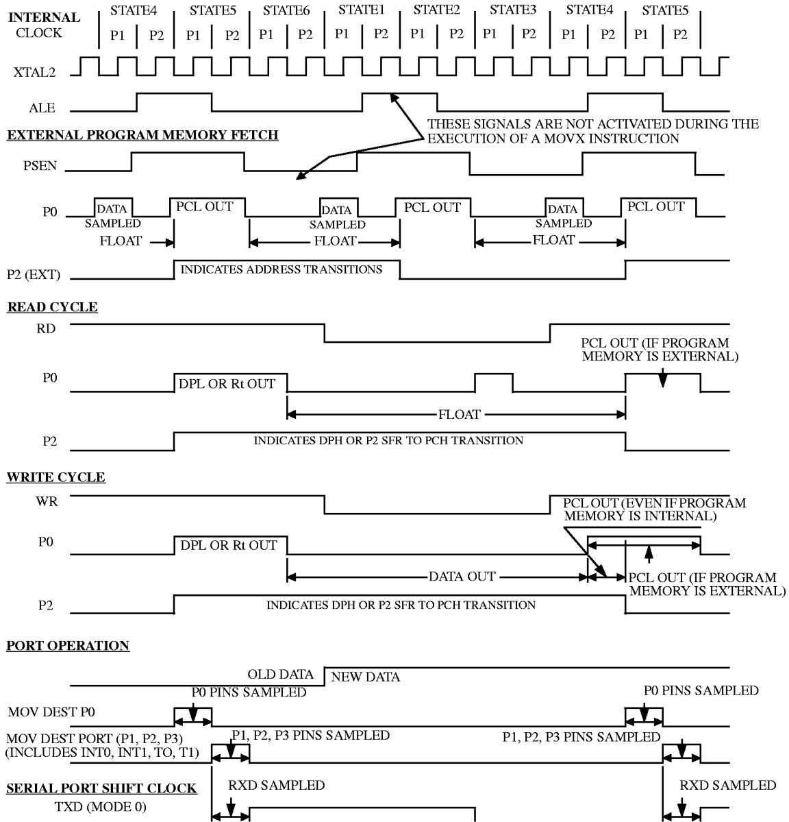
Figure 20. Clock Waveforms
