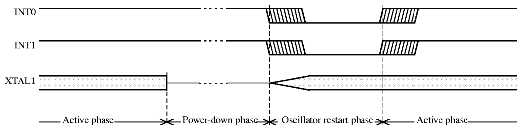
Figure 8. Power-Down Exit Waveform
