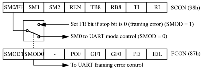
Figure 4. Framing Error Block Diagram
