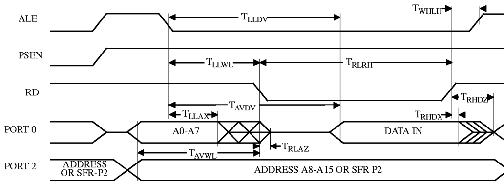
Figure 15. External Data Memory Read Cycle
