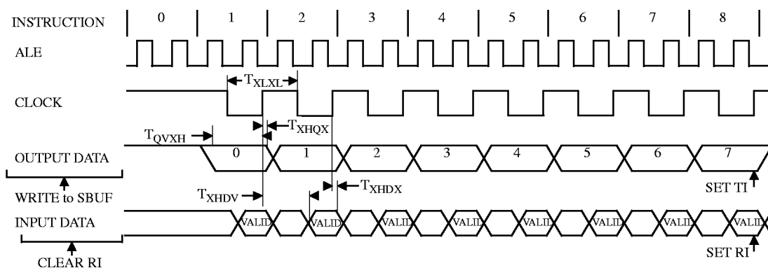
Figure 16. Shift Register Timing Waveforms
