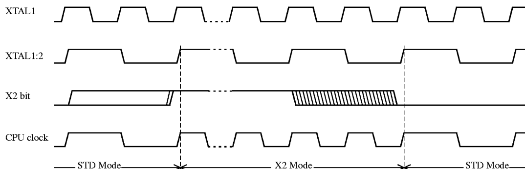
Figure 2. Mode Switching Waveforms
