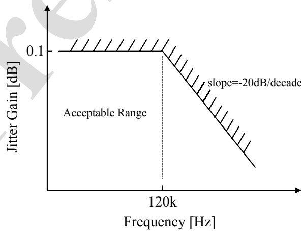
Figure 4.3 Jitter Transfer mask
