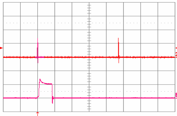
Fig. 27: Load current (top trace, 20 A/div, 20 ms/div) into a 10 mΩ short circuit during restart, at Vin = 48 V. Bottom trace (20 A/div, 1 ms/div) is an expansion of the on-time portion of the top trace.
