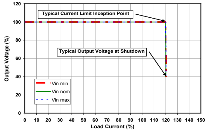
Common Figure 2: Output I-V Characteristics (output voltage vs. load current) showing typical current limit curves and converter shutdown points.
