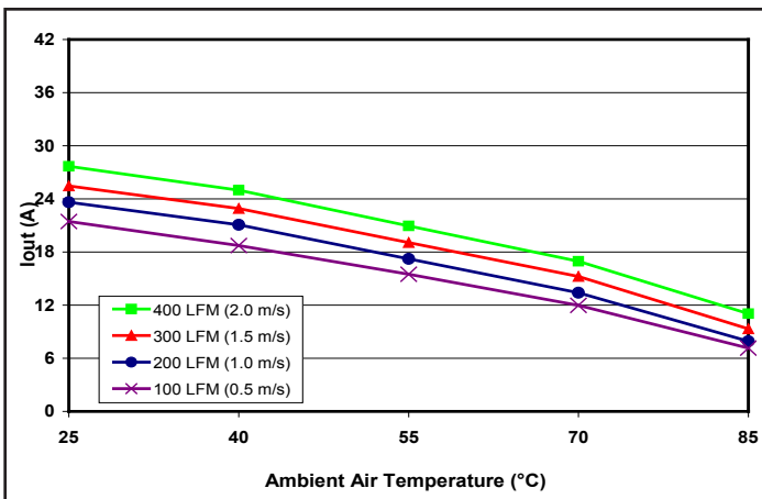
Figure 3: Thermal Derating (max output current vs. ambient air temperature) for encased converter without heatsink, at airflow rates of 100 LFM through 400 LFM. Air flows across the converter from input to output (nominal input voltage).
