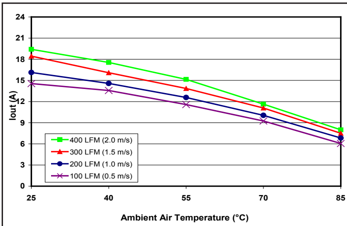
Figure 3: Thermal Derating (max output current vs. ambient air temperature) for encased converter without heatsink, at airflow rates of 100 LFM through 400 LFM. Air flows across the converter from input to output (nominal input voltage).
