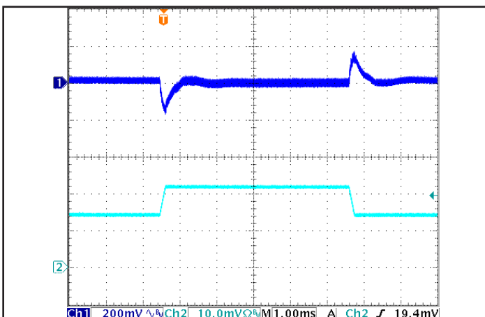
Figure 5: Output Voltage Response to Step-Change in Load Current (50%-75%-50% of Iout(max); dI/dt = 0.2A/μs). Load cap: 15μF tantalum cap and 1μF ceramic cap. Ch 1: Vout, Ch 2: Iout (20A/div).
