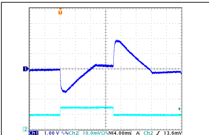
Figure 5: Output Voltage Response to Step-Change in Load Current (50%-75%-50% of I out (max)); dI/dt = 0.1A/μs. Load cap: 100μF electrolytic cap and 1μF ceramic cap. Ch 1: V out , Ch 2: I out (5 A/div).
