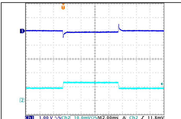
Figure 5: Output Voltage Response to Step-Change in Load Current (50%-75%-50% of I out (max)); dI/dt = 0.1A/μs. Load cap: 15μF tantalum cap and 1μF ceramic cap. Ch 1: V out , Ch 2: I out (20 A/div).
