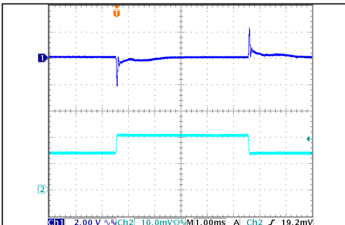
Figure 5: Output Voltage Response to Step-Change in Load Current (50%-75%-50% of Iout(max)); di/dt = 0.1A/\mu s . Load cap: 1 \mu F ceramic cap. Ch 1: Vout, Ch 2: Iout (5 A/div).
