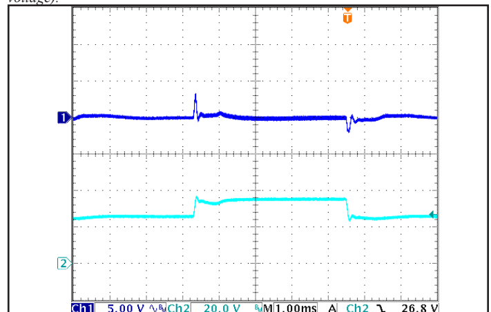
Figure 6: Output Voltage Response to Step-Change in Input Voltage (250 V/ms), at Max. load current. Load cap: 100µF electrolytic cap and 1µF ceramic cap. Ch 1: Vout, Ch 2: Vin.
