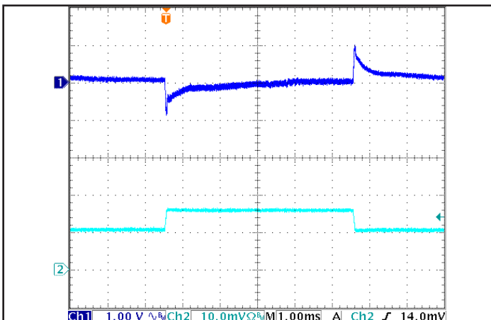
Figure 5: Output Voltage Response to Step-Change in Load Current (50%-75%-50% of Iout(max); dI/dt = 0.1A/us. Load cap: 1µF ceramic cap. Ch 1: Vout, Ch 2: Iout (10 A/div).
