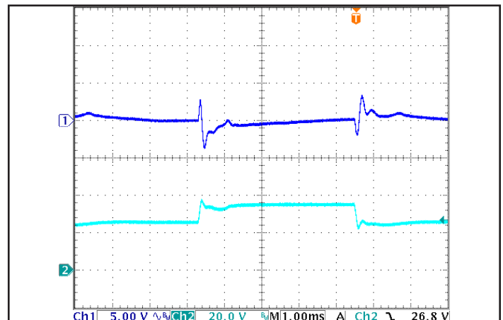
Figure 6: Output Voltage Response to Step-Change in Input Voltage (250 V/ms), at Max. load current. Load cap: 100 \mu F electrolytic cap and 1 \mu F ceramic cap. Ch 1: Vout, Ch 2: Vin.
