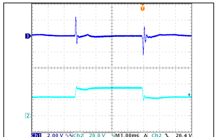
Figure 6: Output Voltage Response to Step-Change in Input Voltage (250 V/ ms), at Max. load current. Load cap: 100μF electrolytic cap and 1μF ceramic cap. Ch 1: V out , Ch 2: V in .
