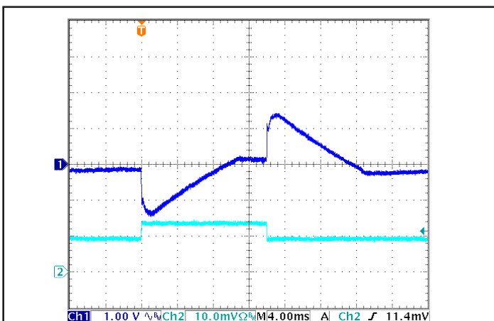
Figure 5: Output Voltage Response to Step-Change in Load Current (50%-75%-50% of I out (max)); dI/dt = 0.1A/μs. Load cap: 100μF electrolytic cap and 1μF ceramic cap. Ch 1: V out , Ch 2: I out (10 A/div).
