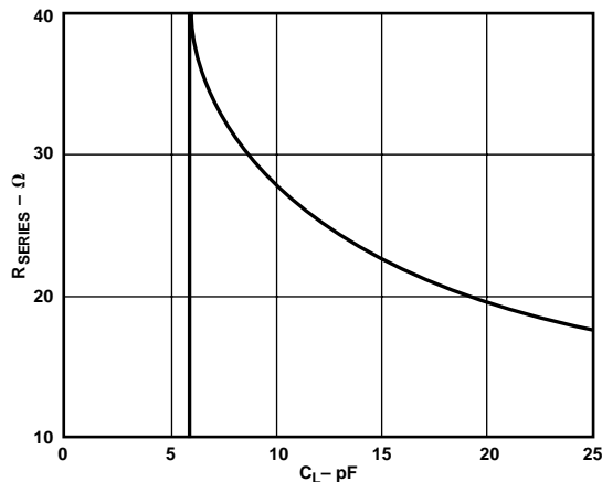
Figure 71. Recommended R_{SERIES} vs. Capacitive Load
