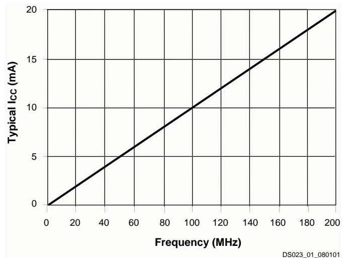
Figure 1: I_{CC} vs. Frequency at V_{CC} = 3.3V, 25^{\circ}C
