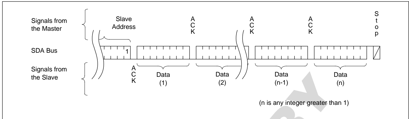
Figure 17. Sequential Read Sequence
