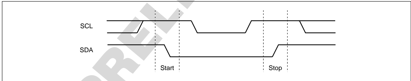
Figure 9. Valid Start and Stop Conditions
