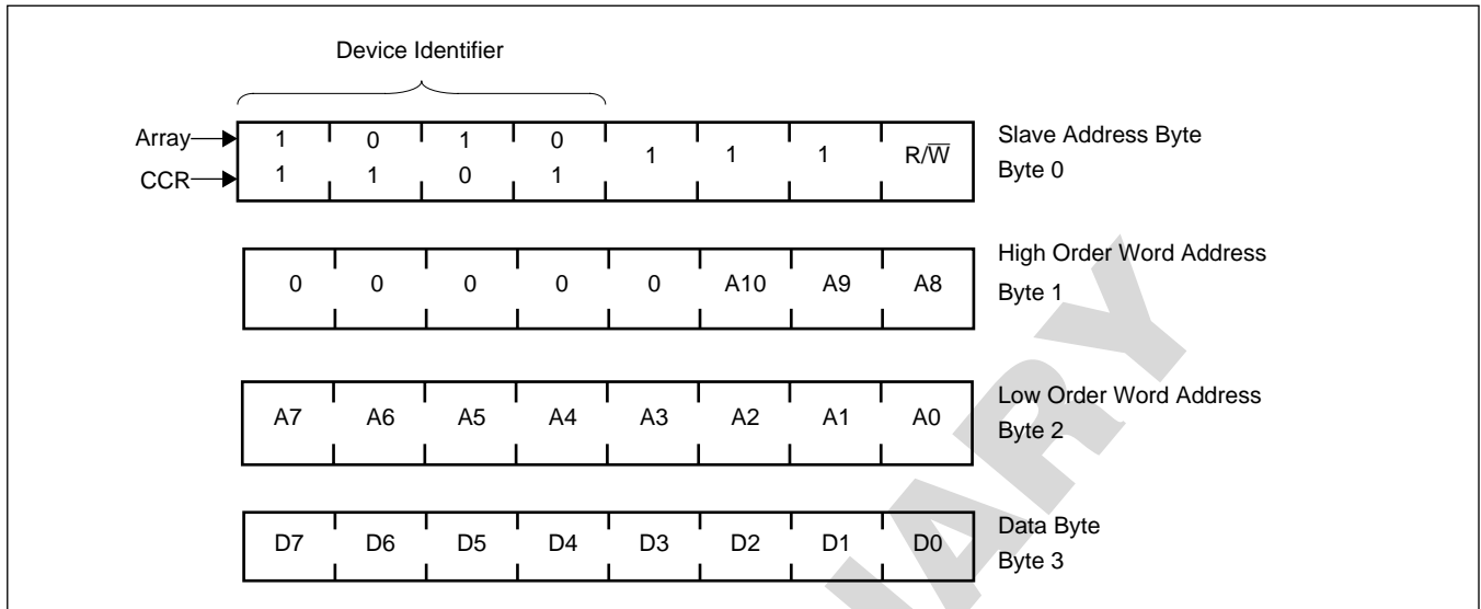
Figure 18. Slave Address, Word Address, and Data Bytes (64 Byte pages)
