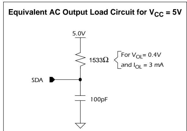
Figure 19. Standard Output Load for testing the device with V_{CC} = 5.0V
