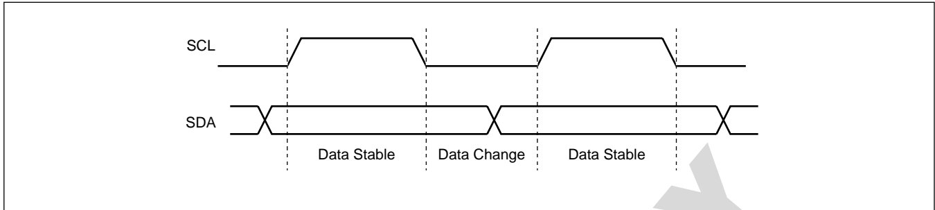
Figure 8. Valid Data Changes on the SDA Bus
