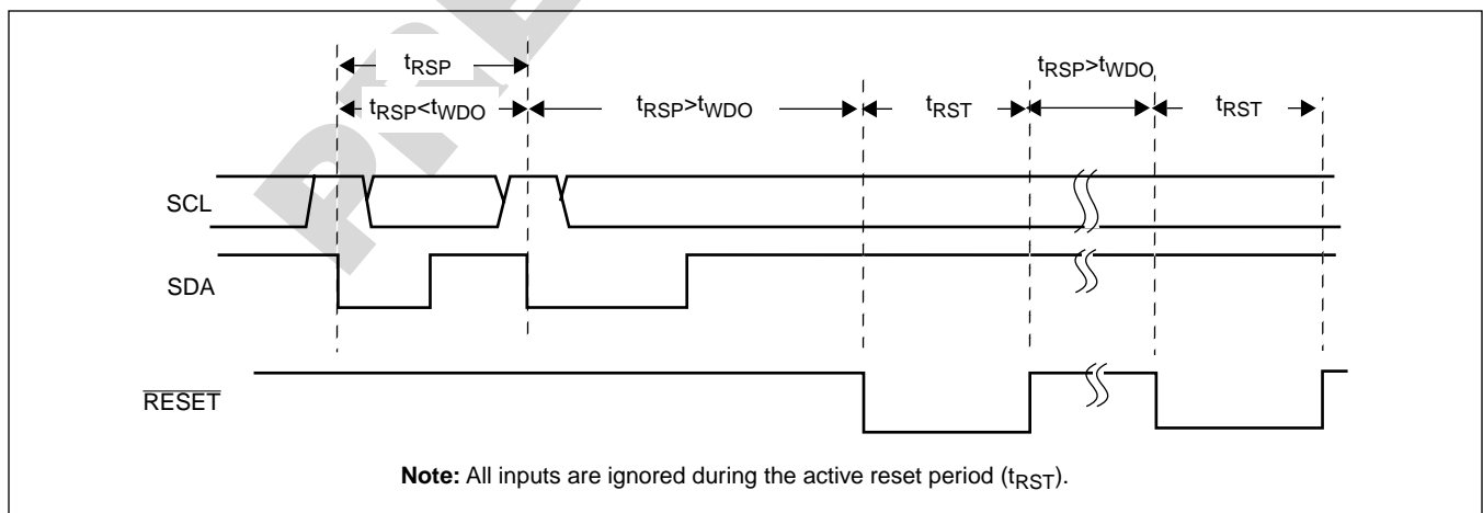
Figure 3. Watchdog Restart/Timeout
