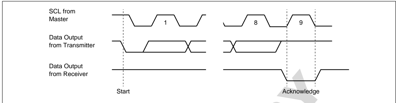
Figure 10. Acknowledge Response From Receiver
