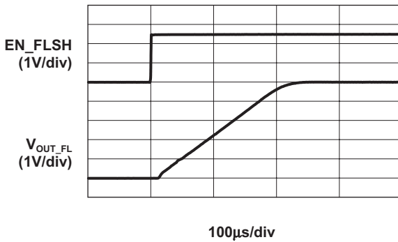
Startup Time (50mA Load)
