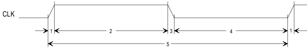
Figure 6: CLK Characteristics
