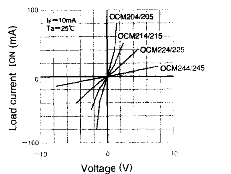
Load current vs. Voltage
