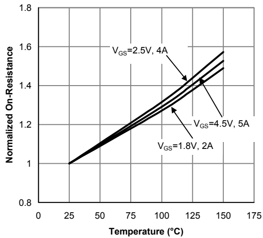
Figure 4: On-Resistance vs. Junction Temperature
