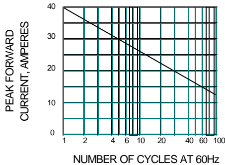
FIG.5 - MAXIMUM NON-REPETITIVE PEAK FORWARD CURRENT
