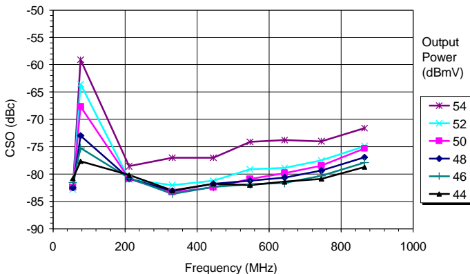
CSO VS. FREQUENCY 128 CHANNEL LOADING, 12dB TILT
