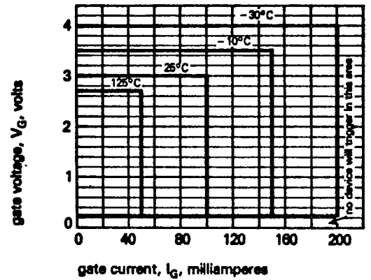
Figure 11 Gate trigger characteristics. Trigger points of all thyristors lie within the areas shown.
