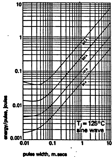
Figure 5 Energy/pulse v. pulse width
