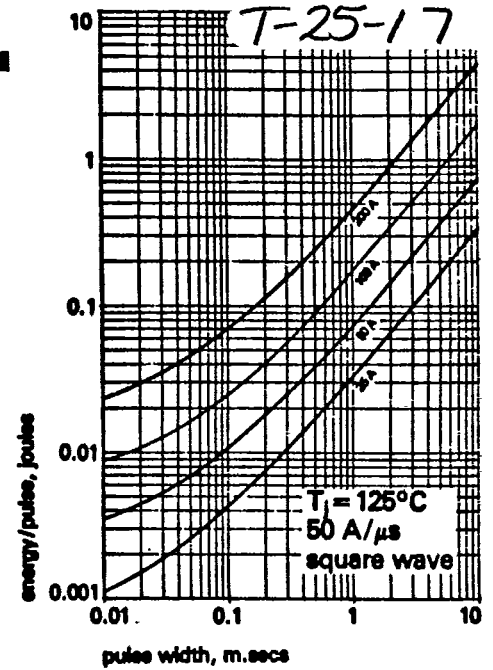
Figure 3 Energy/pulse v. pulse width
