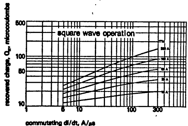
Figure 7 Typical recovered charge at 125°C junction temperature
