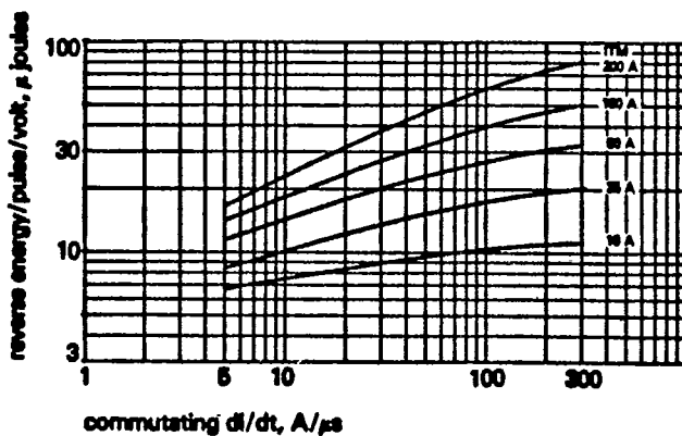
Figure 6 Max. reverse recovery energy loss per pulse at 125°C junction temperature
