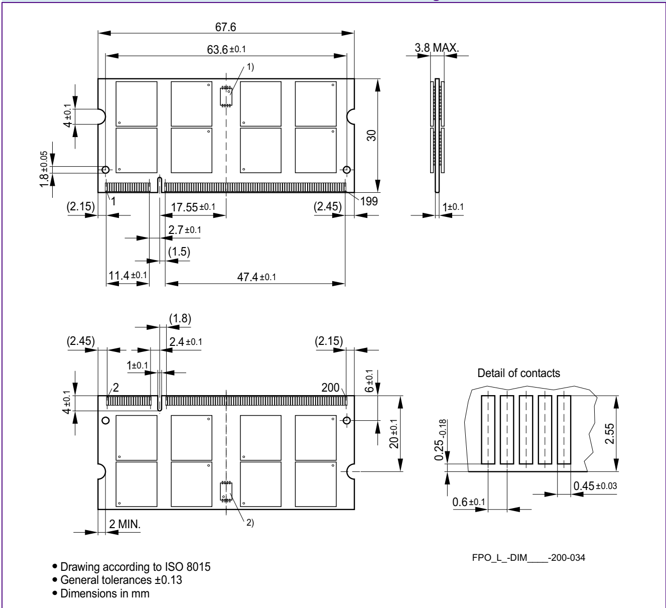
FIGURE 6 Package Outline L-DIM-200-34 Raw Card F
