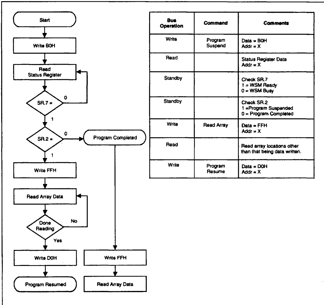
Figure 10. Program Suspend/Resume Flowchart
