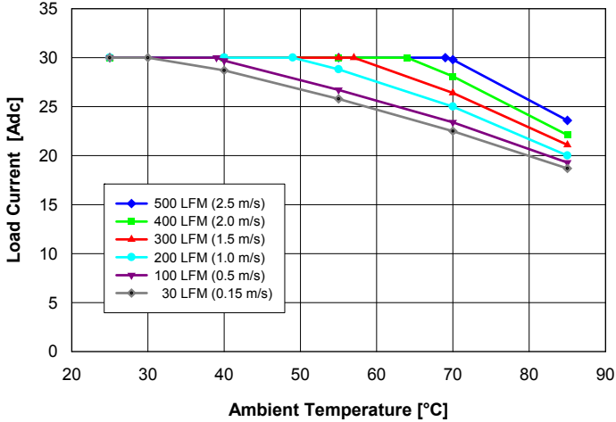
Fig. 12: Available load current vs. ambient temperature and airflow rates for converter mounted horizontally with V_{in} = 27\text{ V} , air flowing from pin 3 to pin 4 and maximum FET temperature \leq 120^{\circ}\text{C} .
