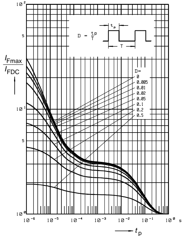
Permissible pulse load I_{Fmax} / I_{FDC} = f(t_p) BAR63-04,-05,-06
