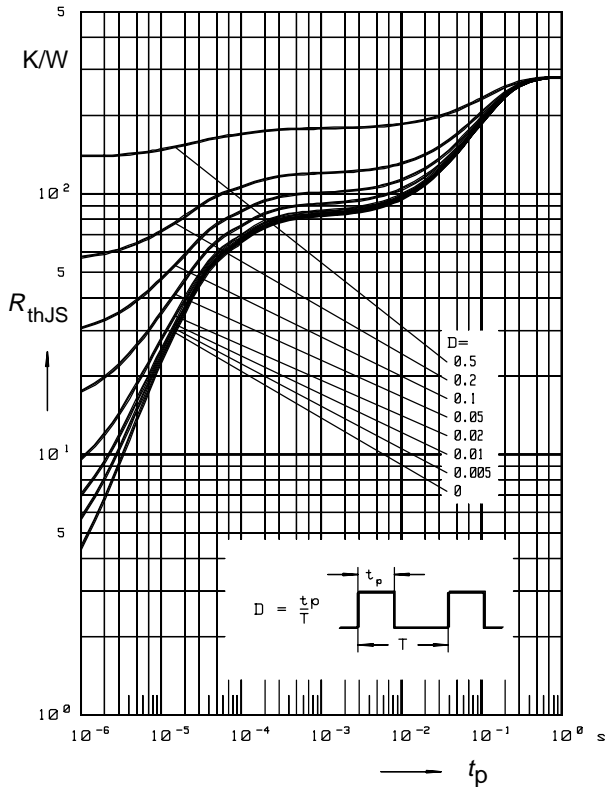
Permissible pulse load R_{thJS} = f(t_p) BAR63-04,-05,-06
