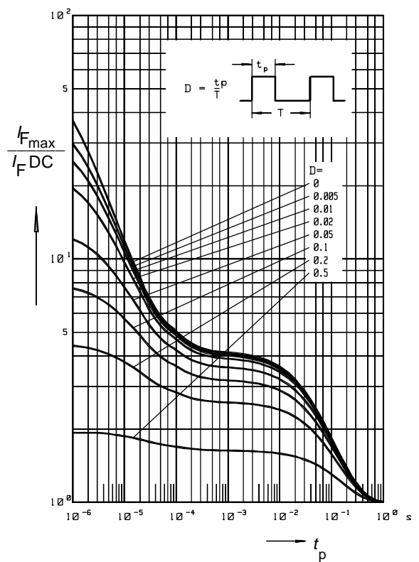
Permissible pulse load I_{Fmax} / I_{FDC} = f(t_p) BAR63-04,-05,-06
