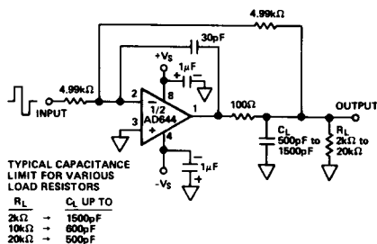
Figure 24. Circuit for Driving a Large Capacitive Load
