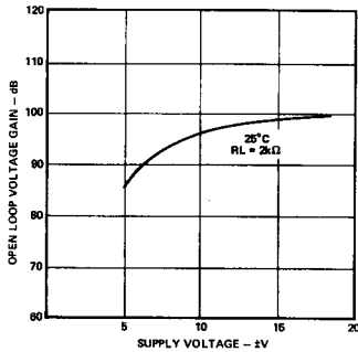
Figure 10. Open Loop Voltage Gain vs. Supply Voltage
