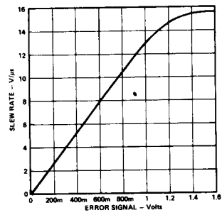
Figure 18. Slew Rate vs. Error Signal
