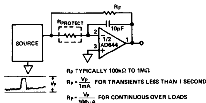
Figure 26. AD644 Input Protection
