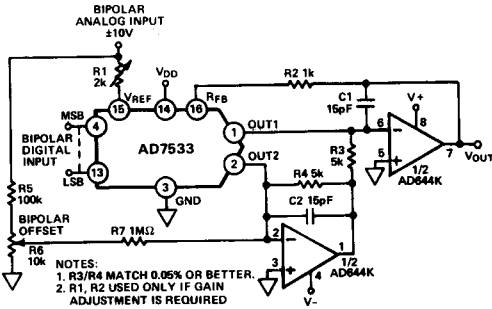
Figure 27a. AD644 Used as DAC Output Amplifiers
