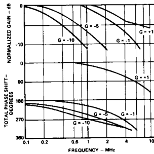
Figure 17. Closed Loop Gain & Phase vs. Frequency
