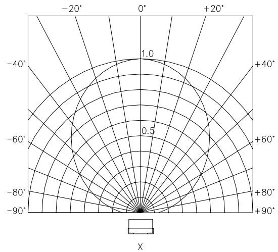
Radiation Diagram
