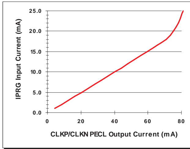
Figure 12: IPRG to CLKP/CLKN Current
