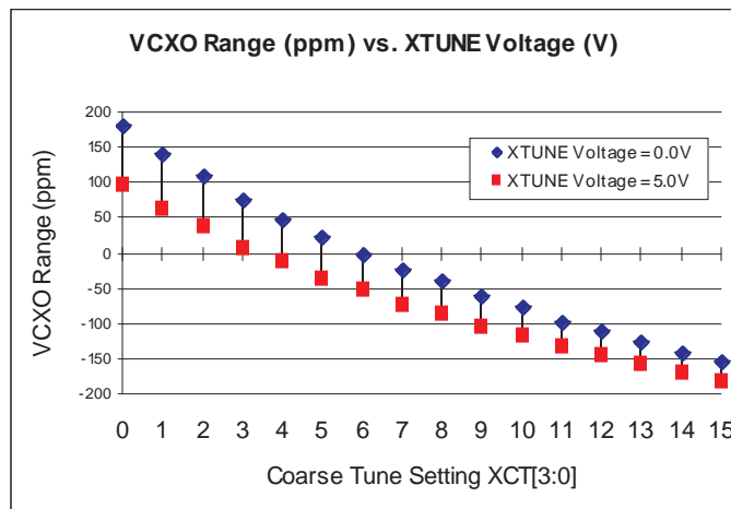
Figure 11: VCXO Coarse and Fine Tuning
