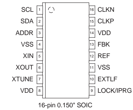
Figure 1: Pin Configuration
