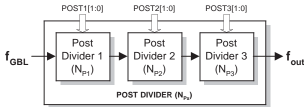
Figure 4: Post Divider
