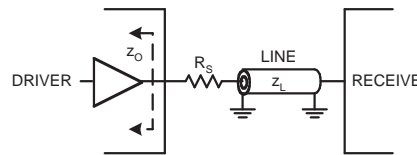
Figure 23: Series Termination (CMOS)
