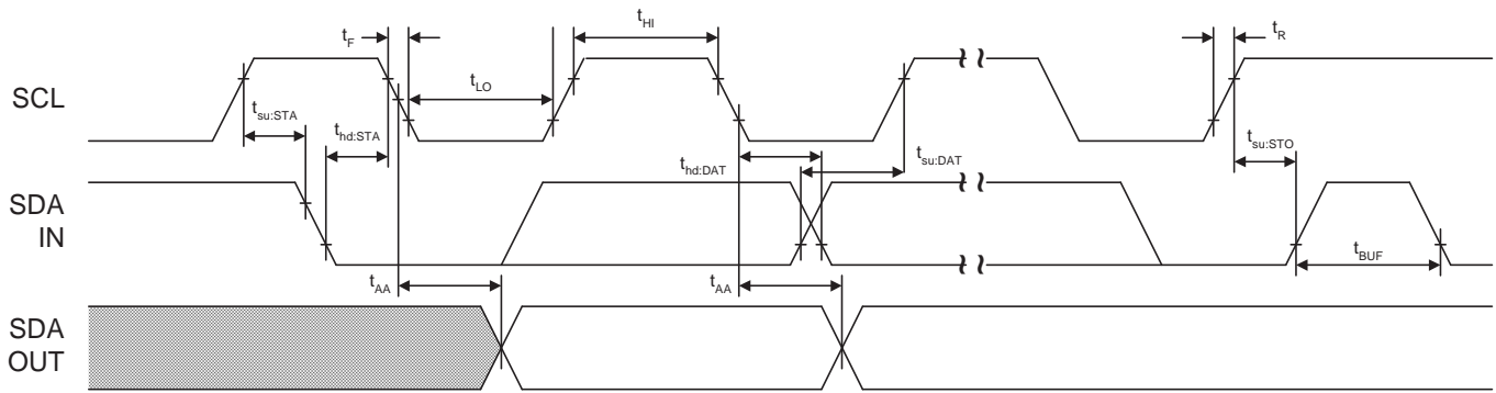
Figure 18: Data Transfer Sequence
