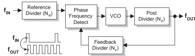
Figure 7: Aligned I/O Phase
