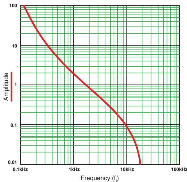
Figure 8: Loop Gain vs. Frequency
