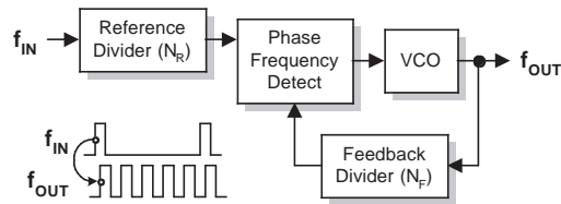
Figure 5: Simple PLL
