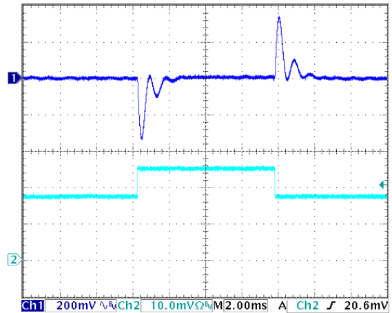
Figure 16: Output voltage response to step-change in load current (50%-75%-50% of I_{out(max)} ; dI/dt = 5A/\mu s ). Load cap: 470 \mu F , 30m \Omega ESR tantalum cap and 1 \mu F ceramic cap. Ch 1: V_{out} (200mV/div), Ch 2: I_{out} (2A/div).
