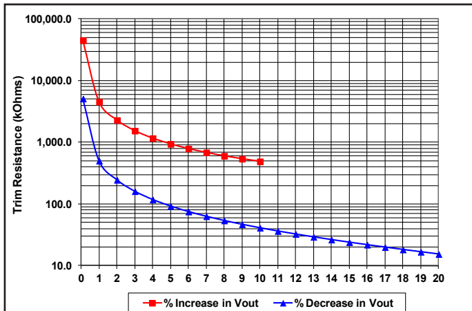
Figure C: Trim Graph
