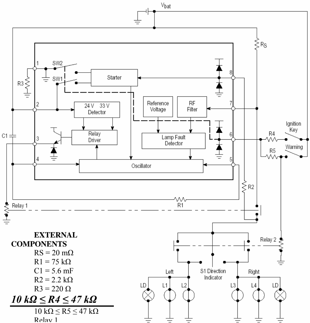
Figure 10. Typical IL33193 Application
