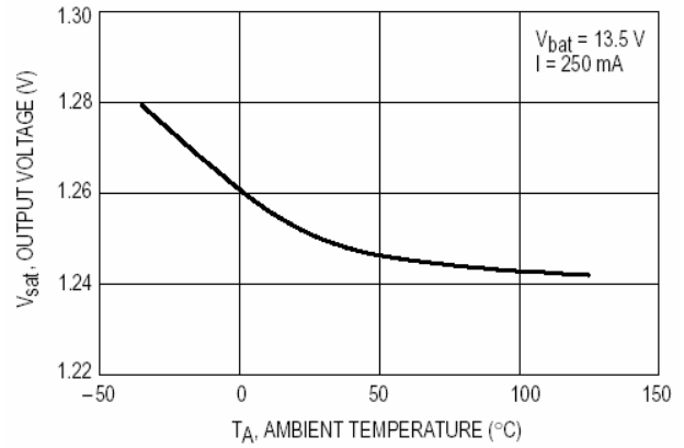
Figure 6. Output Voltage versus Temperature
