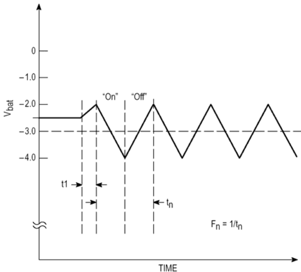
Figure 1. Normal Operation Oscillator Timing Diagram
