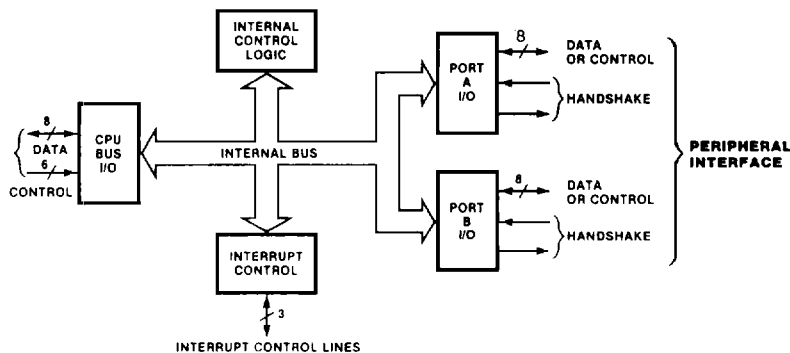
Figure 4. Block Diagram
