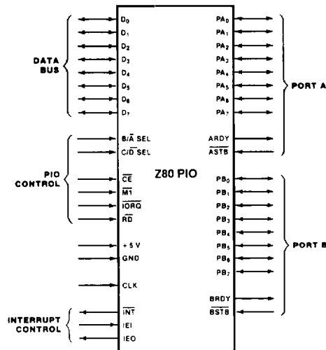
Figure 1. Pin Functions
