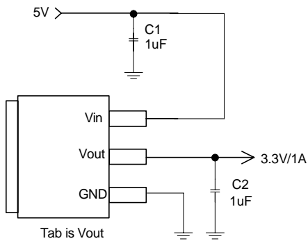
( 5V/3.3V fixed output )
