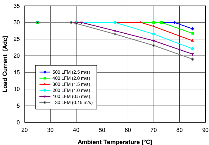
Fig. 1: Available load current vs. ambient air temperature and air flow rates for Q48T30020 converter mounted vertically with air flowing from pin 3 to pin 1, MOSFET temperature \leq 120^{\circ}\text{C} , V_{in} = 54\text{ V} .
