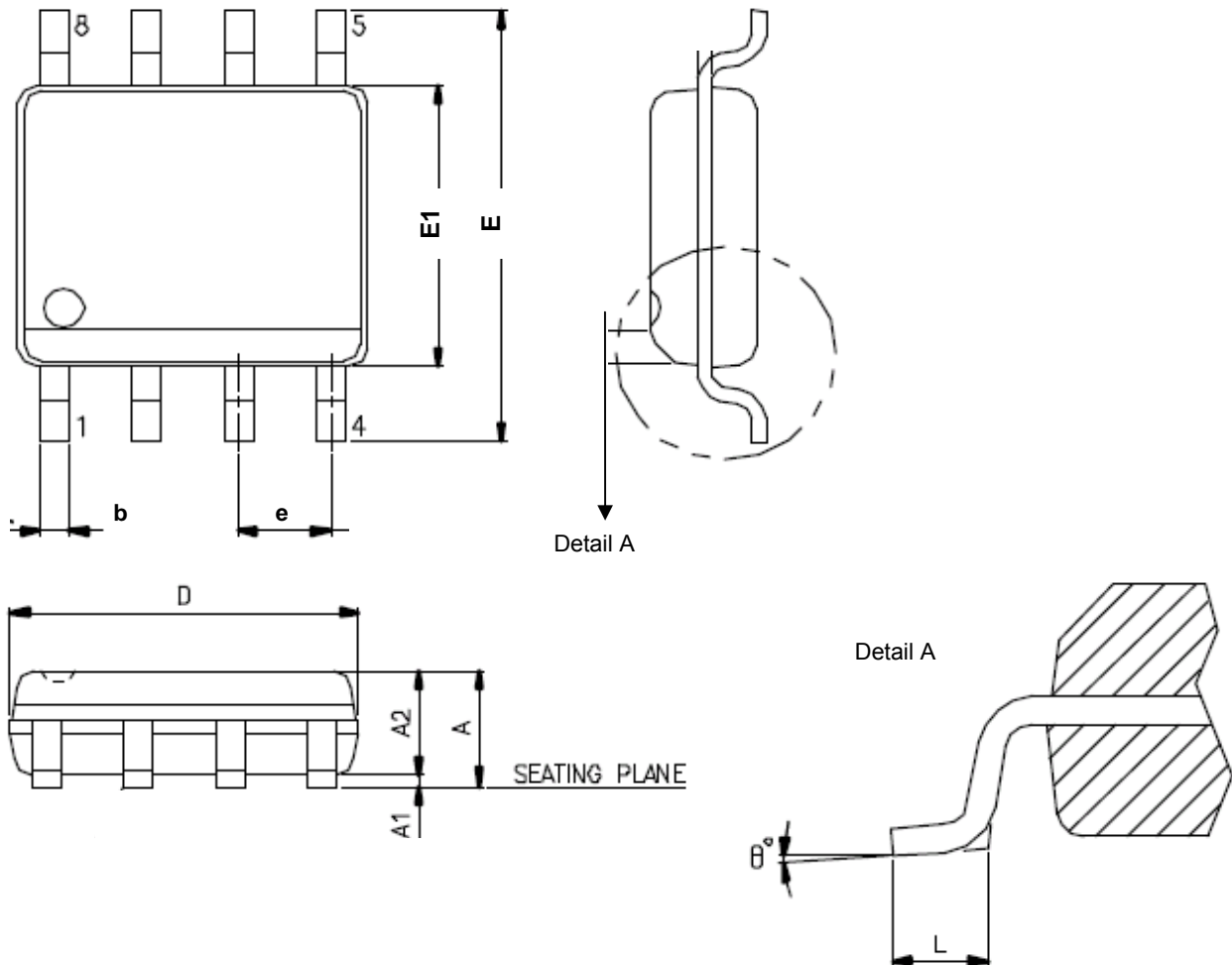
Figure 24. SOP 8 ( 150 mil )
