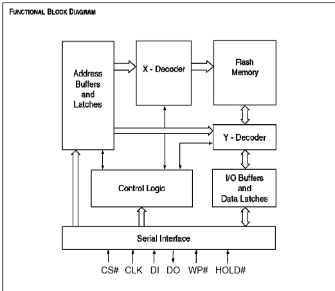
Figure 2. BLOCK DIAGRAM
