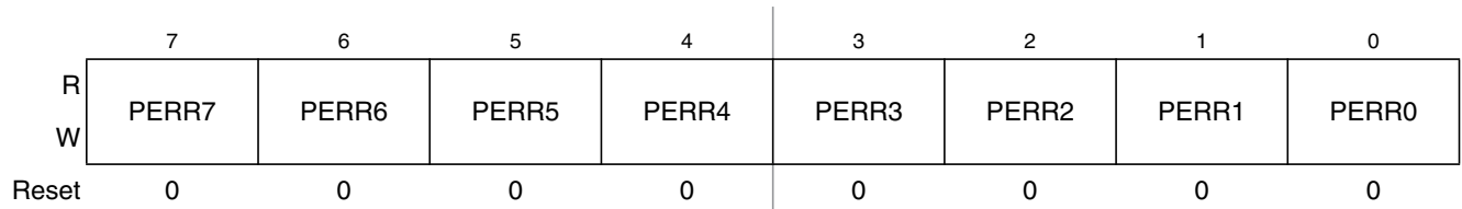
Figure 2-87. Port R Pull Device Enable Register (PERR)
