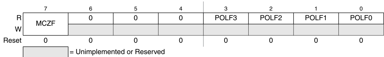
Figure 14-42. 16-Bit Modulus Down-Counter FLAG Register (MCFLG)
