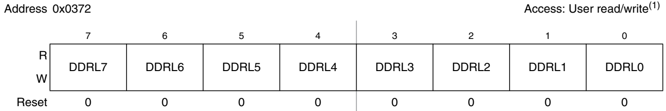
Figure 2-93. Port L Data Direction Register (DDRL)
