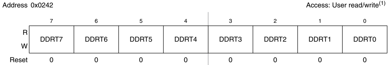
Figure 2-21. Port T Data Direction Register (DDRT)
