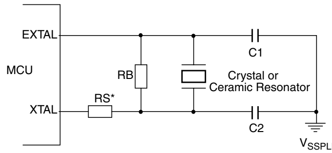
Figure 12-3. Full Swing Pierce Oscillator Connections (FSP mode selected)
