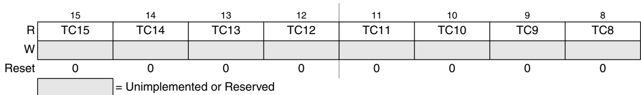
Figure 14-58. Timer Input Capture Holding Register 0 High (TC0H)
