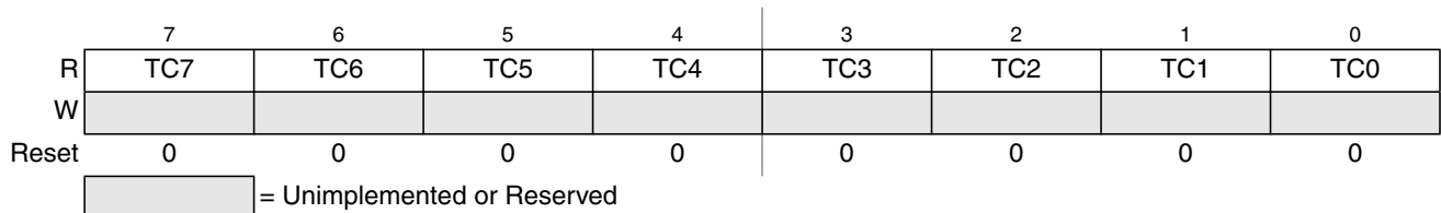
Figure 14-59. Timer Input Capture Holding Register 0 Low (TC0L)
