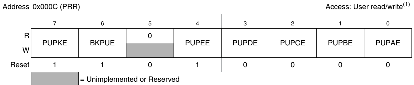
Figure 2-11. S12X_EBI ports, BKGD pin Pull-up Control Register (PUCR)
