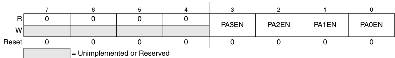
Figure 14-43. Input Control Pulse Accumulators Register (ICPAR)
