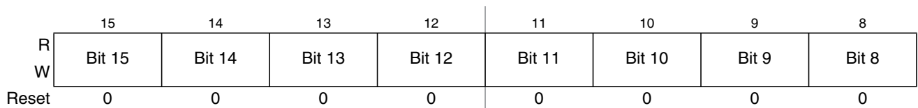
Figure 14-23. Timer Input Capture/Output Compare Register 2 High (TC2)
