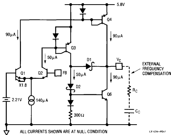
Figure 10. Error Amplifier
