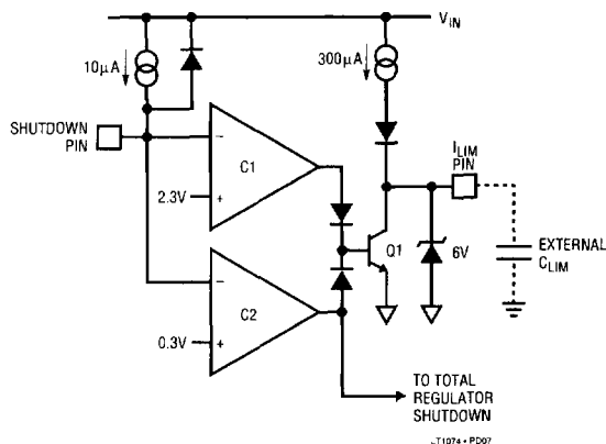
Figure 5. Shutdown Circuitry
