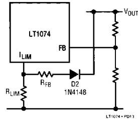
Figure 9. Foldback Current Limit
