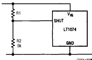
Figure 6. Undervoltage Lockout
