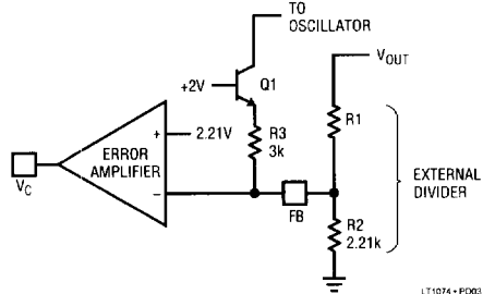
Figure 3. Frequency Shifting
