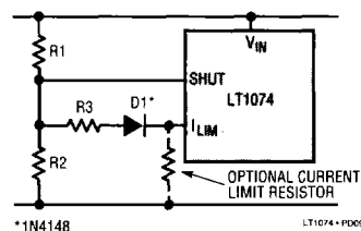
Figure 7. Adding Hysteresis
