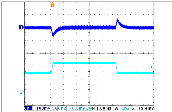
Figure 5: Output voltage response to step-change in load current (50% -75% -50% of I out (max); dl/dt = 0.1 A/μs). Load cap: 15 μF Tantalum + 1 μF Ceramic capacitor. Ch 1: V out , Ch 2: I out (20 A/div).
