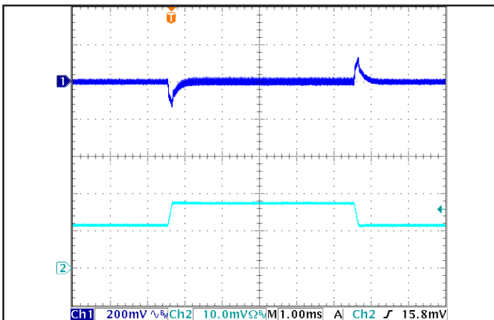
Figure 5: Output voltage response to step-change in load current (50% -75% -50% of I out(max) ; dI/dt = 0.1 A/μs). Load cap: 15 μF Tantalum + 1 μF Ceramic capacitor. Ch 1: V out , Ch 2: I out (20 A/div).
