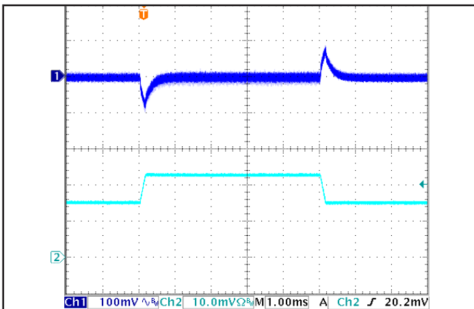
Figure 5: Output voltage response to step-change in load current (50% -75% -50% of I_{out(max)} ; dI/dt = 0.1 A/\mu s ). Load cap: 15 \mu F Tantalum + 1 \mu F Ceramic capacitor. Ch 1: V_{out} , Ch 2: I_{out} (20 A/div).
