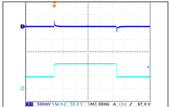
Figure 6: Output voltage response to step-change in input voltage (1000 V/ms). Load cap: 15 \mu F Tantalum + 1 \mu F Ceramic capacitor. Ch 1: V_{out} , Ch 2: V_{in} .
